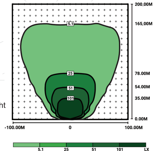
Light plot for GP125K at 6.5m
