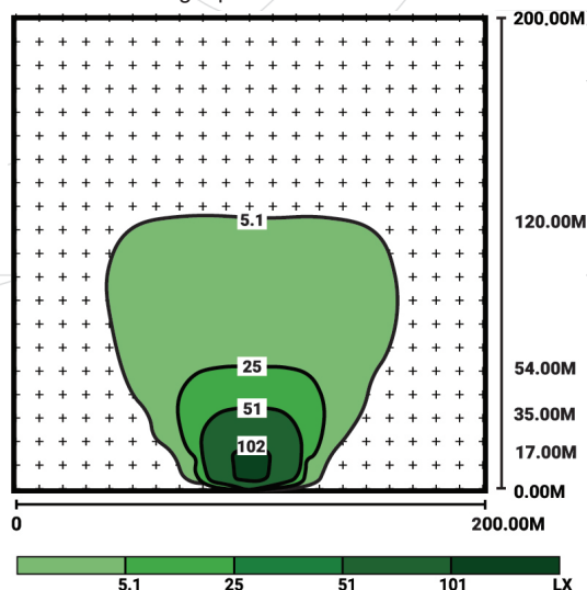
Light plot for GP65K at 9m
